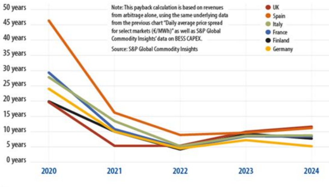
Payback period – four hour LFP BESS
